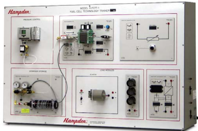
The Model H-FCTT-1 Fuel Cell Technology Trainer allows the student to create a grid independent power supply that uses only hydrogen as its fuel.
